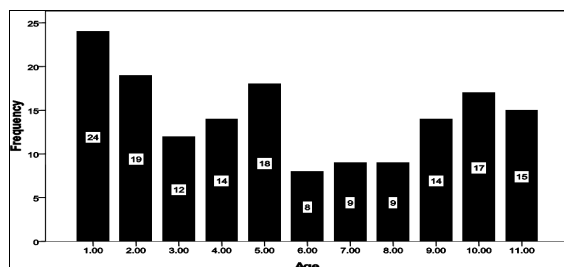
Figure-1: Frequency distribution of age
